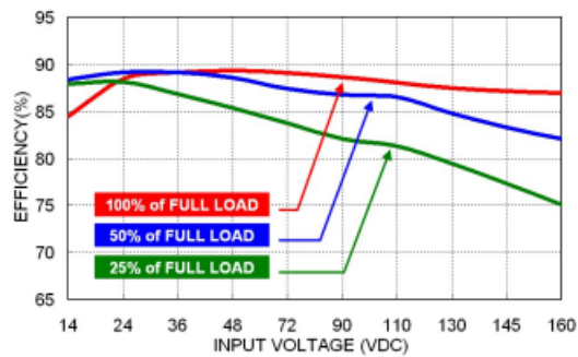
43QAE40-72S05U Efficiency vs. Input Voltage
