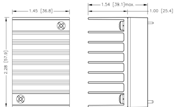
43QAE40-□□S□□U –HS5 7GA0125P01-F
