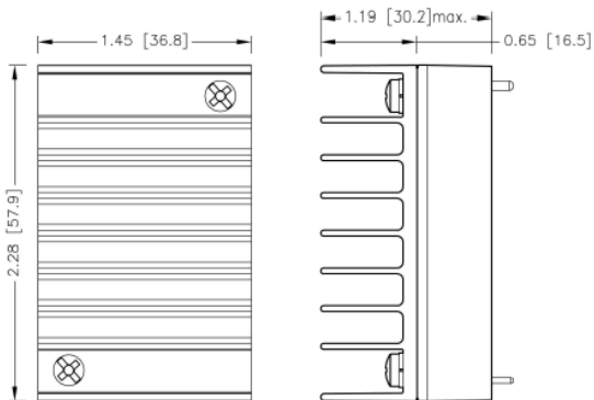
43QAE40-□□S□□U –HS4 7GA0124P01-F
