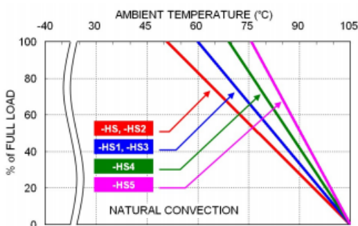
43QAE40-72S05U Derating Curve with Heat-sink (See Thermal Considerations)
