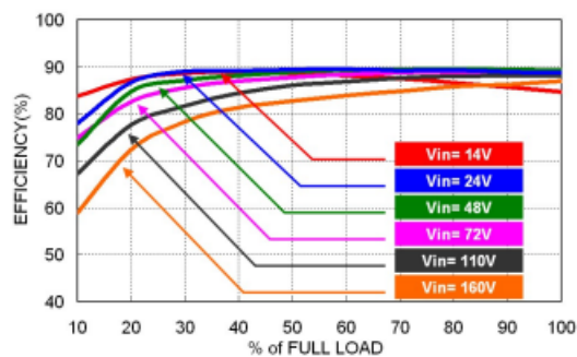
43QAE40-72S05U Efficiency vs. Output Load
