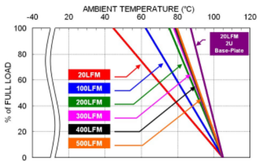
43QAE40-72S05U Derating Curve (See Thermal Considerations)
